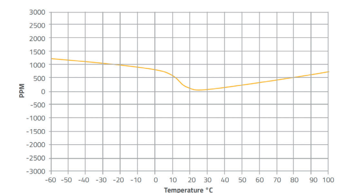
Typical Phase Change vs. Temperature Low Loss PTFE Cables
