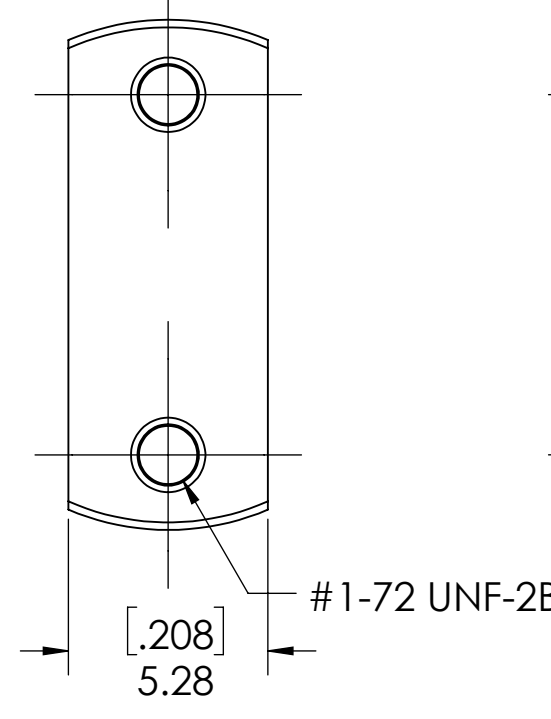
LOCKING BLOCK
