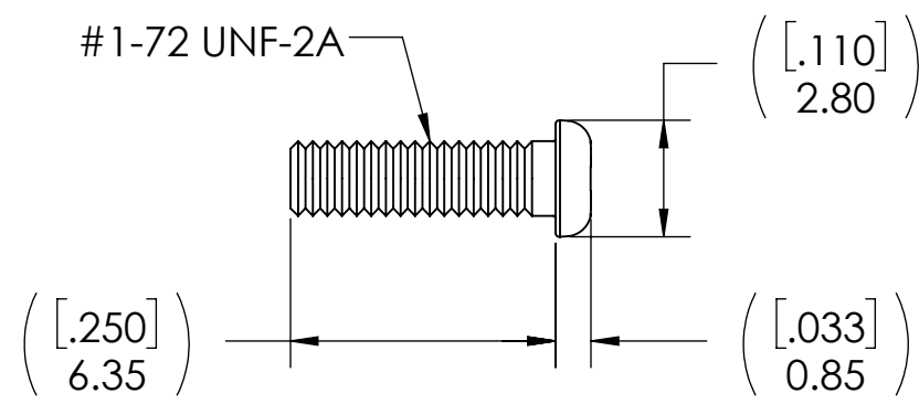
SCREW
