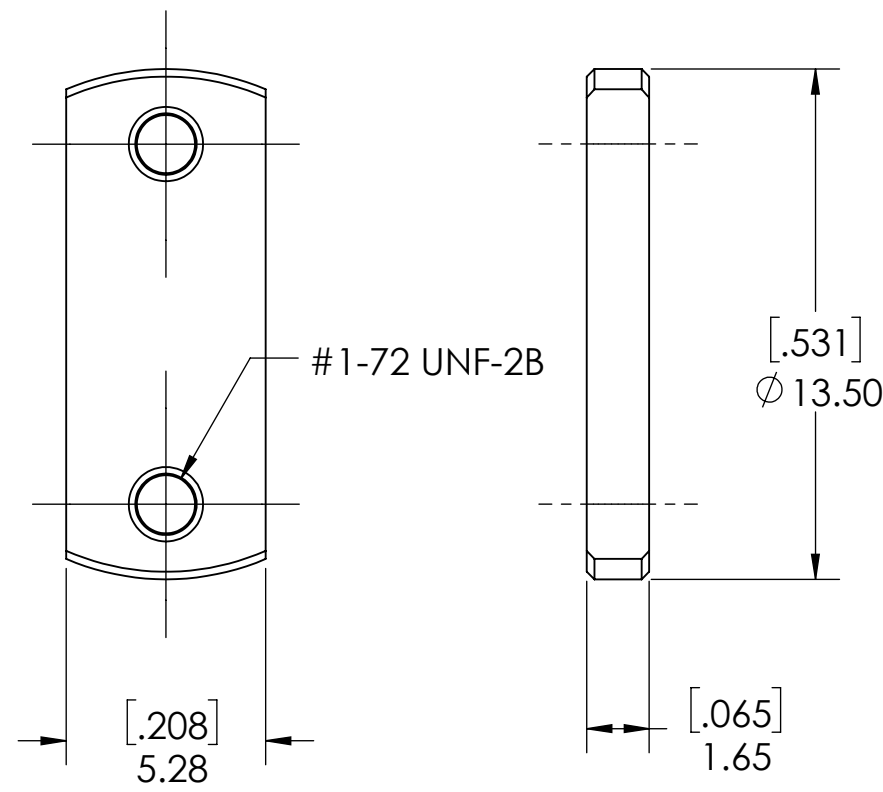
LOCKING BLOCK
