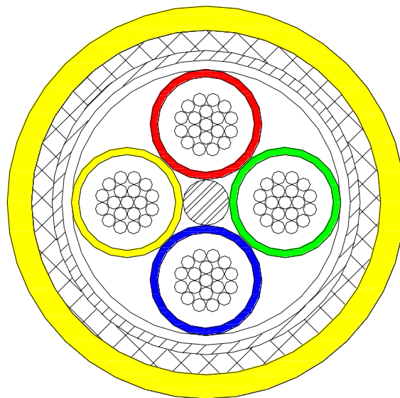
NF24Q100-01HP Cable Cross Section
