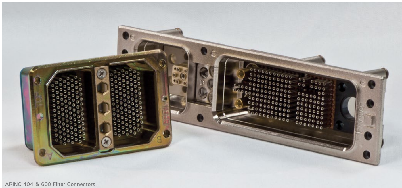
ARINC 404 & 600 Filter Connectors
