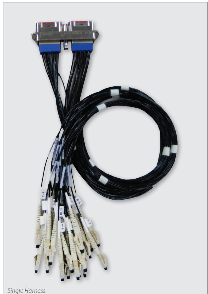
Test Adapter Interface
