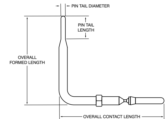
PC Right-Angle Contact
