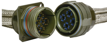
Terminated Assemblies with a Pair of Size 19 38999 Connectors
